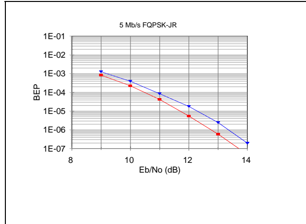
Figure A-21. FQPSK-JR BEP vs. E_b/N_0 .
