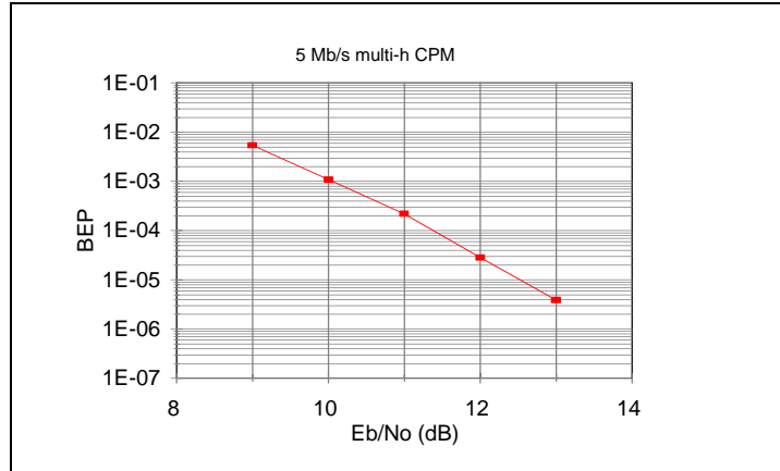
Figure A-26. BEP versus E_b/N_0 performance of 5 Mb/s ARTM CPM.
