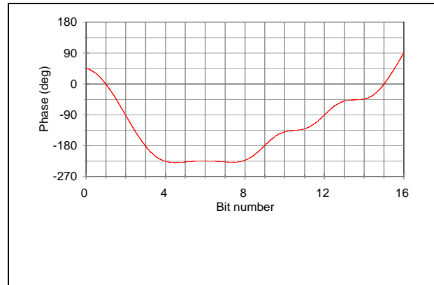
Figure A-22. Measured SOQPSK-TG phase trajectory
