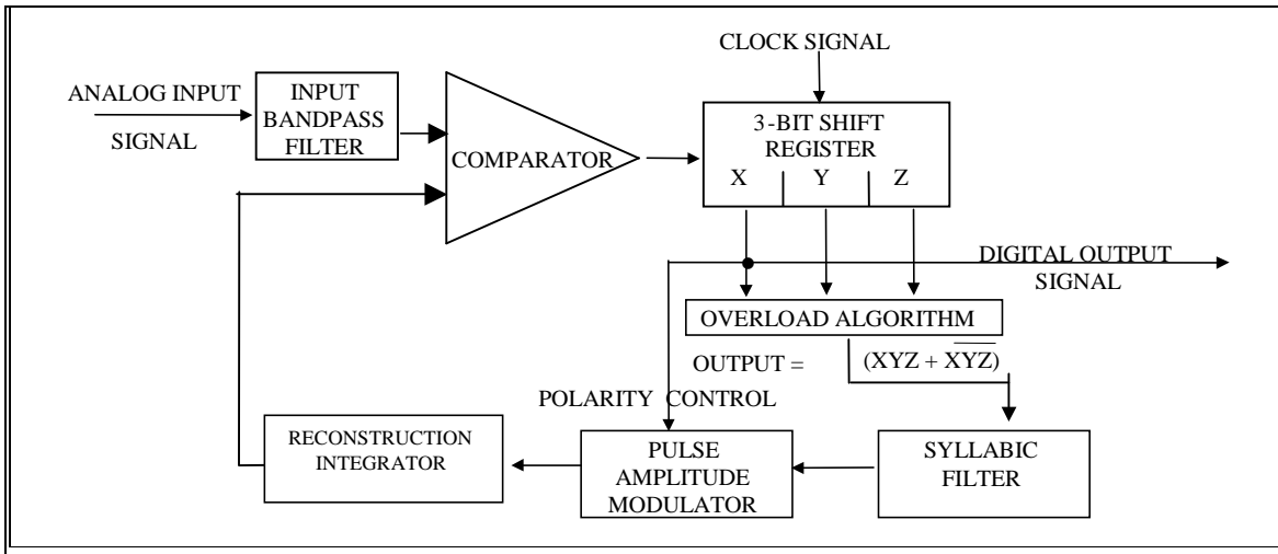
Figure F-1a. Typical CVSD encoder.
