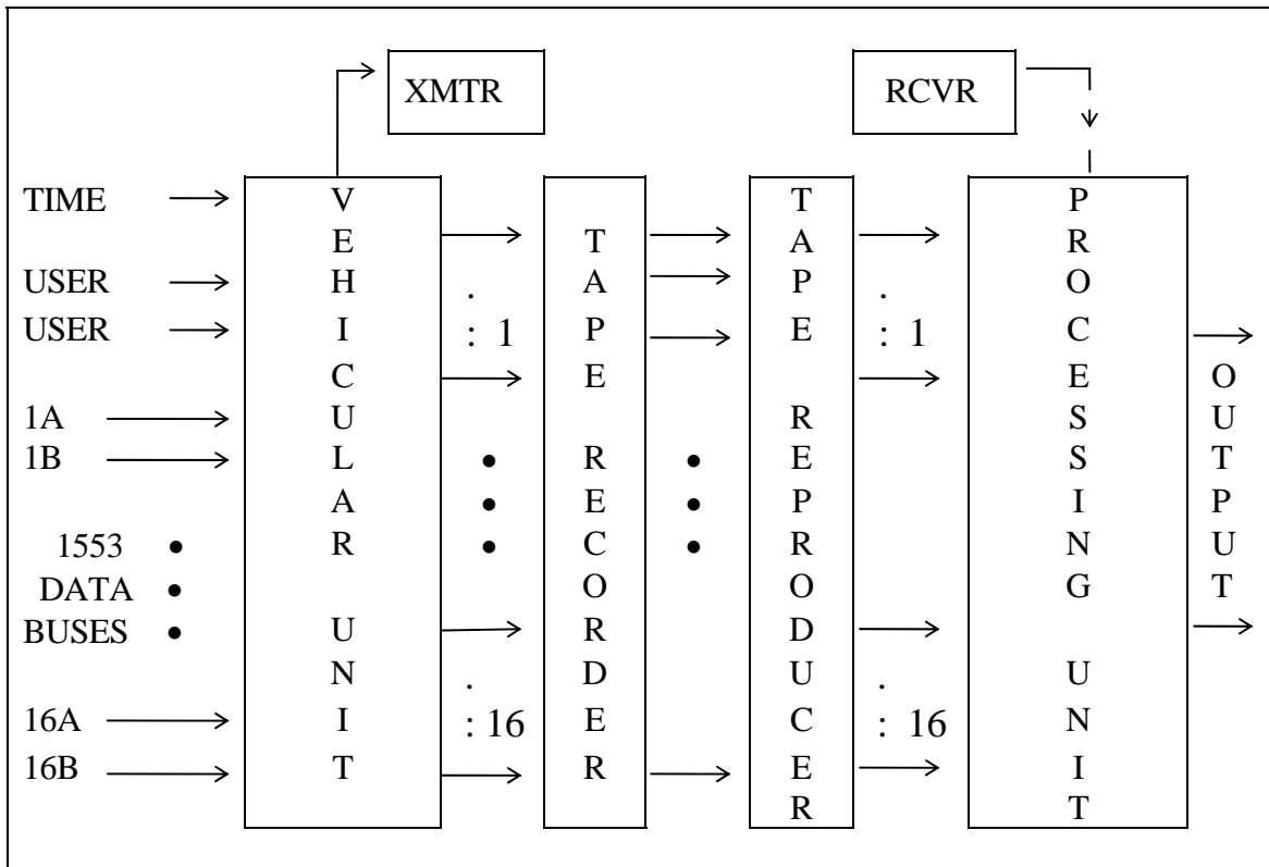
Figure 8-4. System block diagram.
