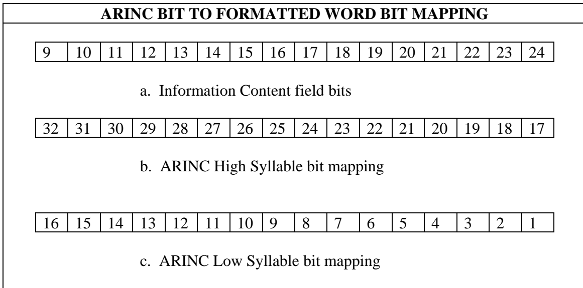
Figure 8-7. ARINC bit to formatted word bit mapping.
