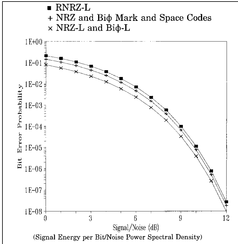
Figure A-3. Theoretical BEP Performance for Various Baseband PCM Signaling Techniques (Perfect Bit Synchronization Assumed)
