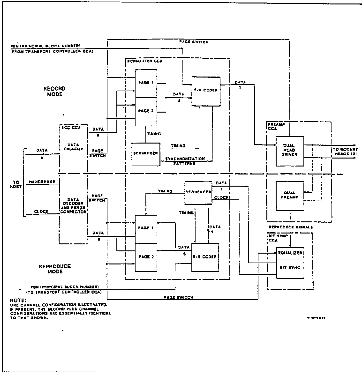
Figure 6-15. Typical VLDS data path electronics block diagram.
