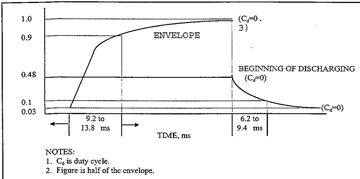
Figure F-2. Typical envelope characteristics of the decoder output signal for CVSD.
