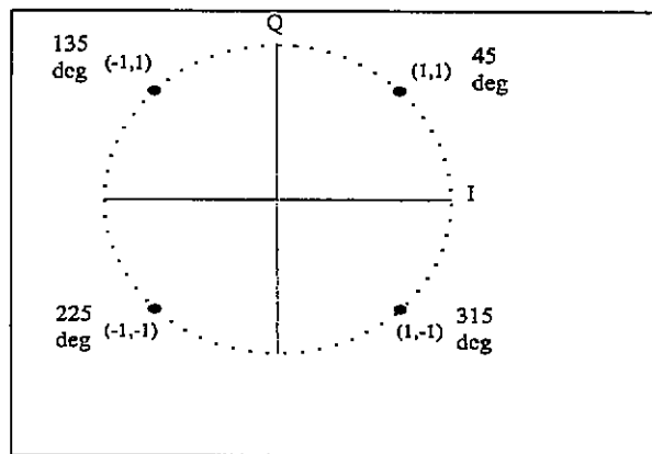
Figure A-11. I & Q constellation.
