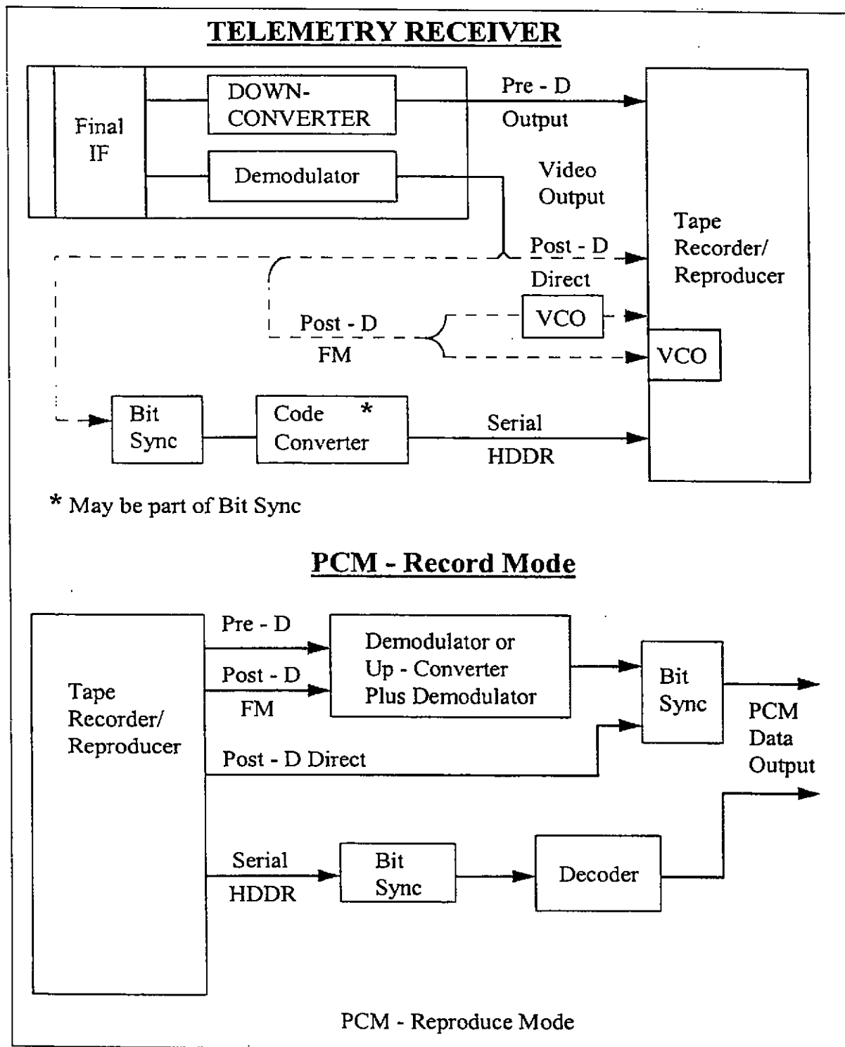
Figure 6-4. PCM record and reproduce configuration.
