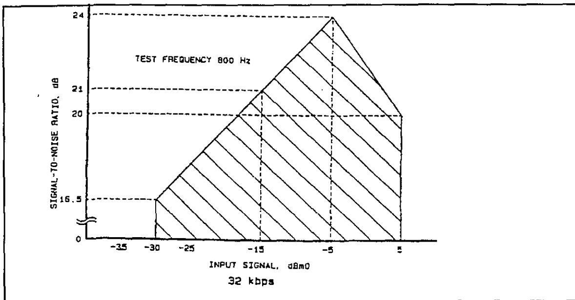
Figure F-6b. Signal to quantizing noise ratio versus input level for CVSD (32 kbps).
