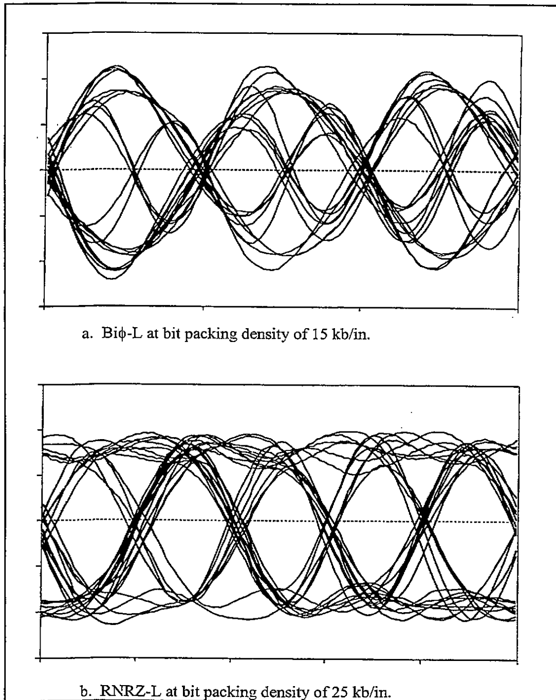
Figure D-5. Sample eye patterns at output of recorder/reproducer.
