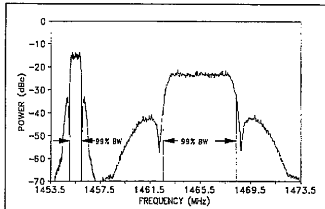
Figure A-1. 800-kb/s and 5-Mb/s RNRZ PCM/FM signals.
