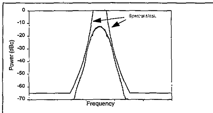
Figure A-9. Typical 1-Mb/s FQPSK-B signal and spectral mask.
