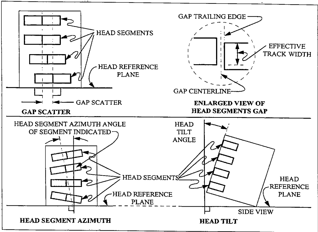
Figure 6-3. Head and head segment mechanical parameters.
