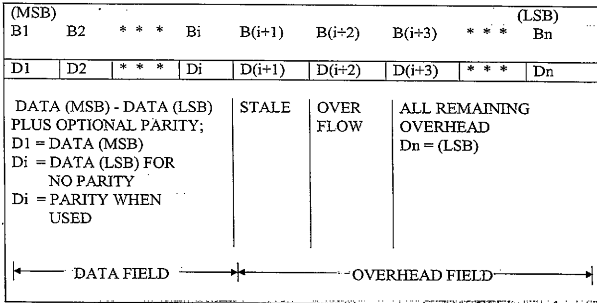
Figure 4-5. Asynchronous word structure.
