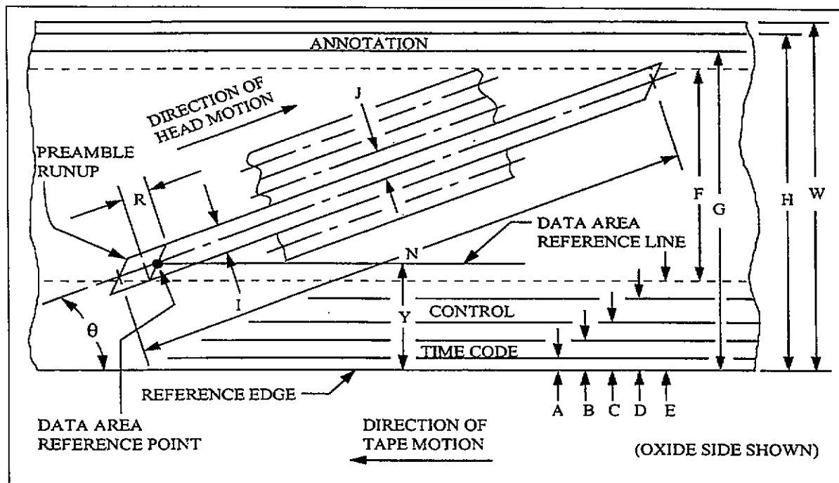
Figure 6-6. Location and dimensions of recorded tracks.
