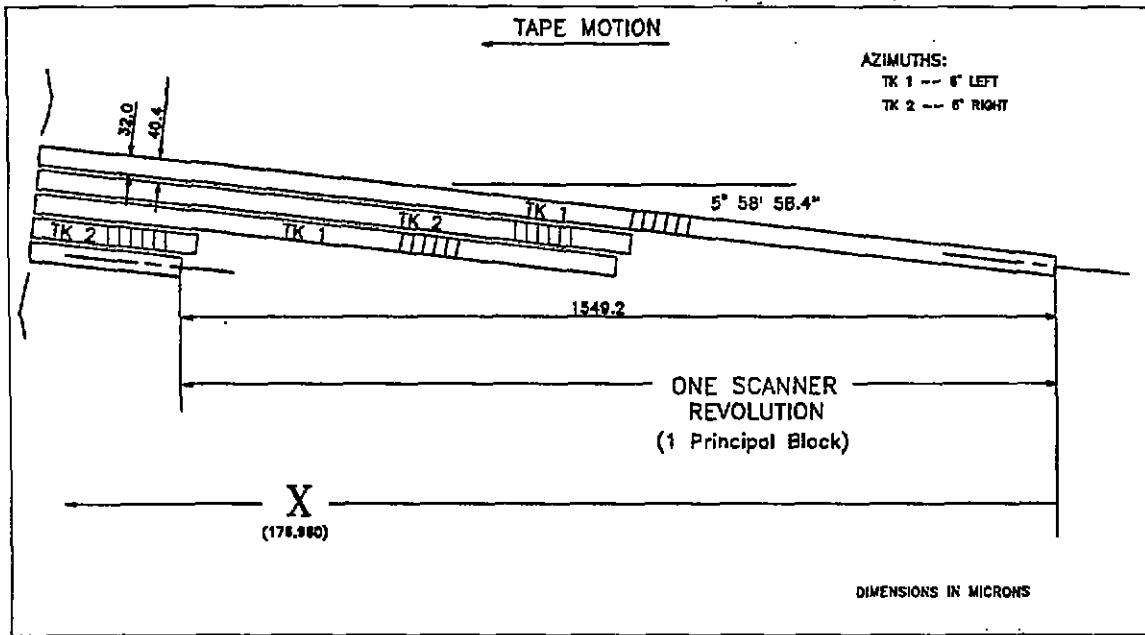
Figure 6-10. Helical track dimensions, B format.
