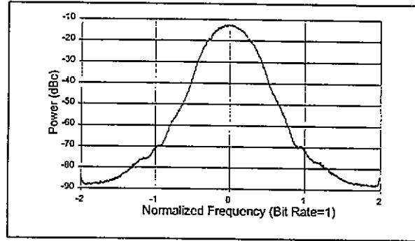
Figure A-15. FQPSK-B spectrum with random input data.
