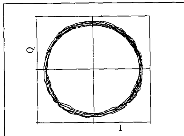
Figure A-14. FQPSK-B vector diagram.
