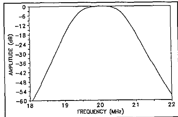
Figure A-6. Typical receiver IF filter response (-3 dB bandwidth = 1 MHz).
