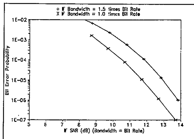
Figure C-1. BEP versus IF SNR in bandwidth = bit rate for NRZ-L PCM/FM.
