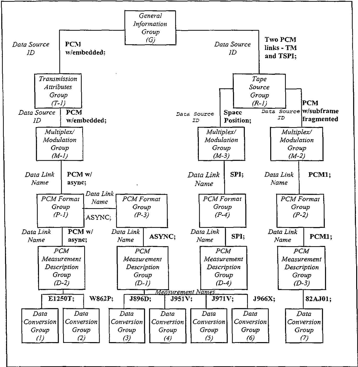
Figure J-1. Group linkages.
