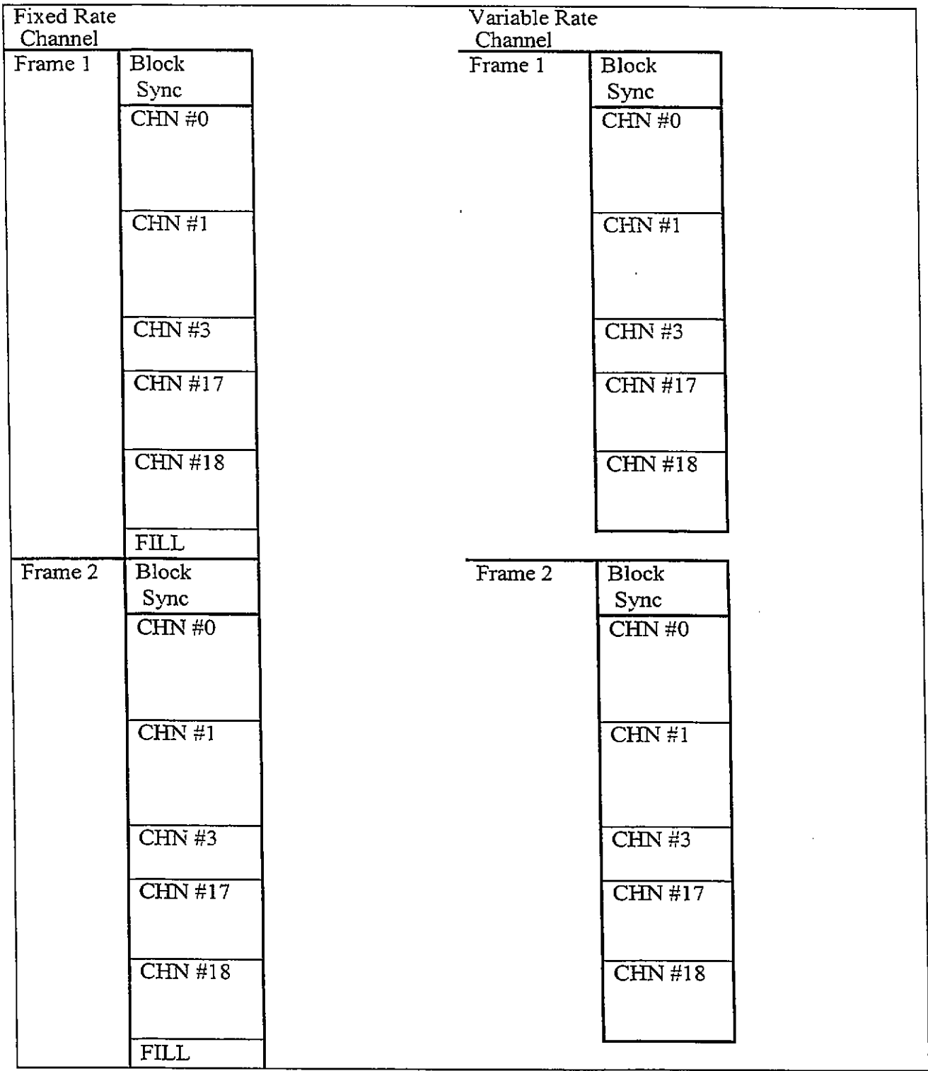
Figure G-5. Submux aggregate format.
