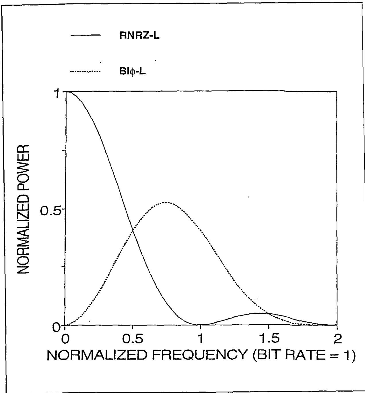
Figure D-4. Random PCM power spectra.
