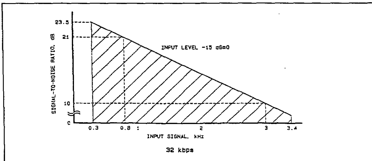
Figure F-7b. Signal to quantizing noise ratio versus frequency for CVSD (32 kbps).
