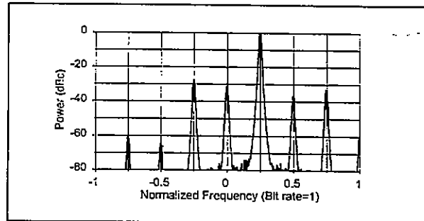
Figure A-16. FQPSK-B spectrum with all 1's input and large modulator errors.
