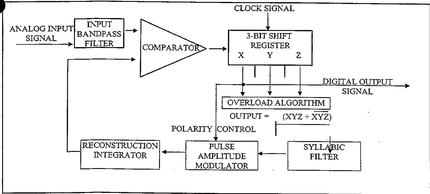
Figure F-1a. Typical CVSD encoder.
