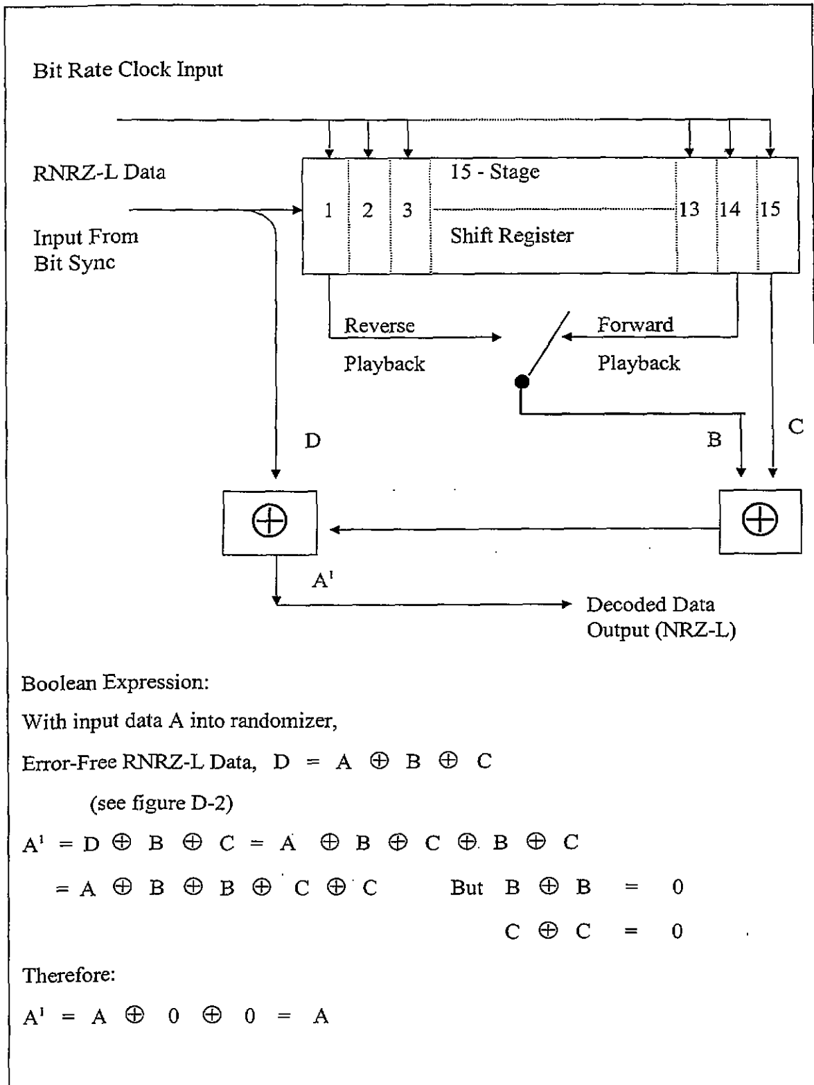
Figure D-3. Randomized NRZ-L decoder block diagram.
