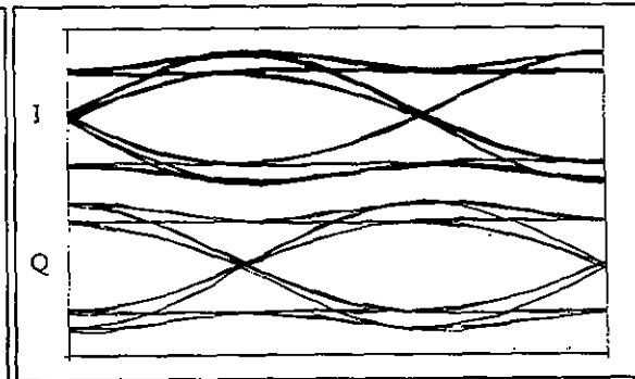
Figure A-13. FQPSK-B I & Q eye diagrams (at input to IQ modulator).
