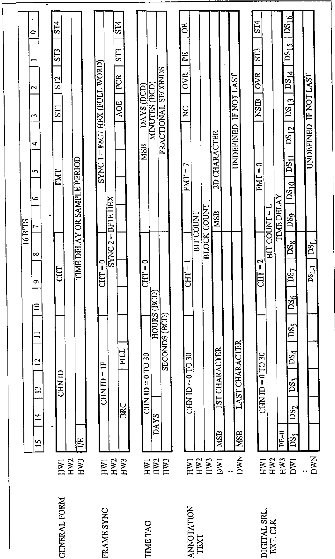
Figure 6-9a. Submux data format.
