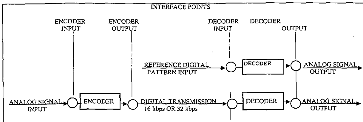
Figure F-3. Interface diagram for CVSD converter.
