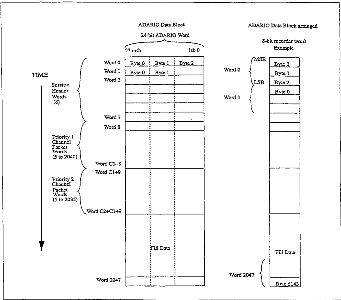
Figure G-2. ADARIO data blocks.
