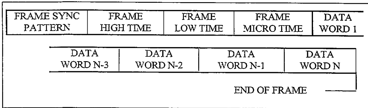
Figure 8-3. Composite frame structure.
