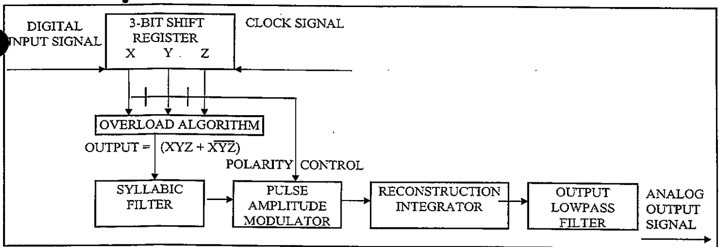
Figure F-1b. Typical CVSD decoder.
