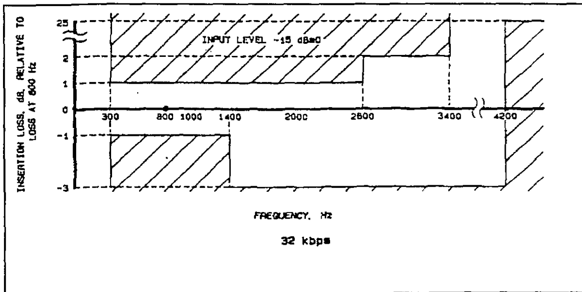
Figure F-4b. Insertion loss versus frequency for CVSD (32 kbps).
