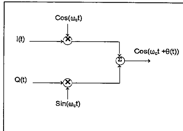
Figure A-10. OQPSK modulator.
