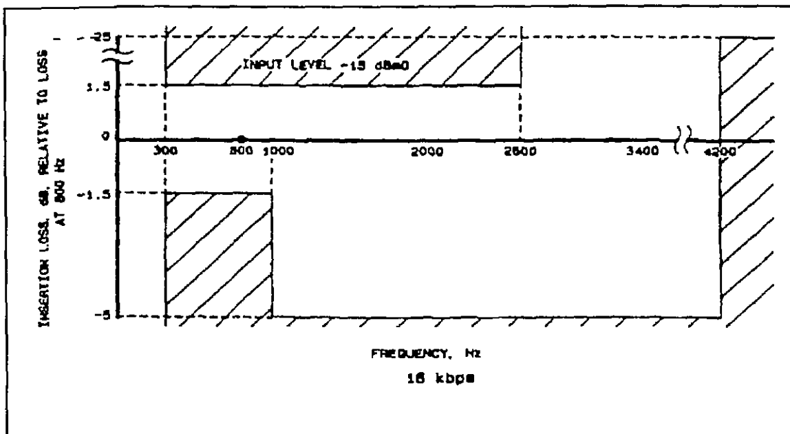
Figure F-4a. Insertion loss versus frequency for CVSD (16 kbps).
