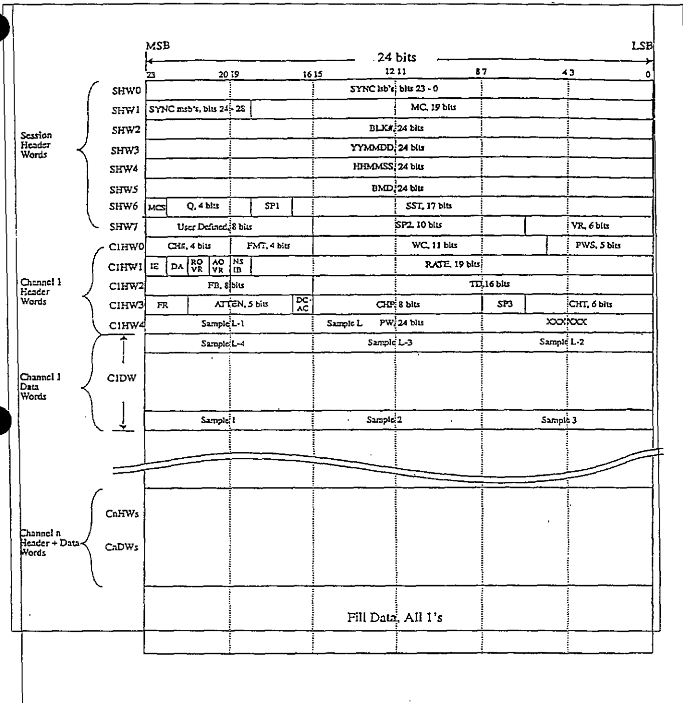
Figure G-1. ADARIO data format.
