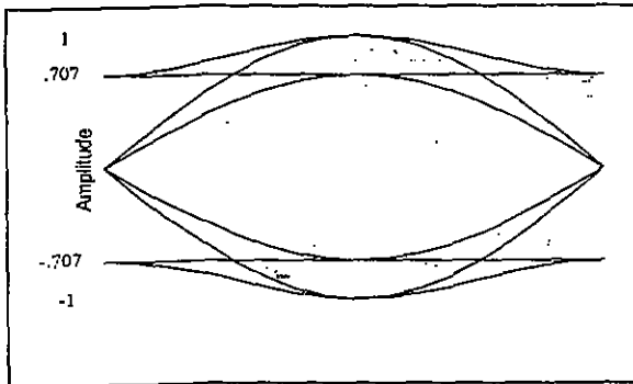
Figure A-12. FQPSK-B wavelets.
