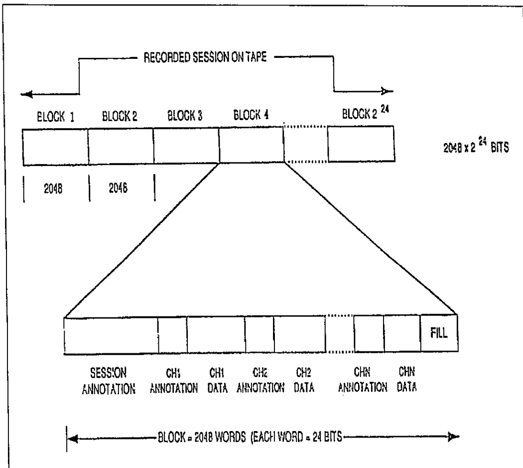
Figure 6-7. ADARIO block format.
