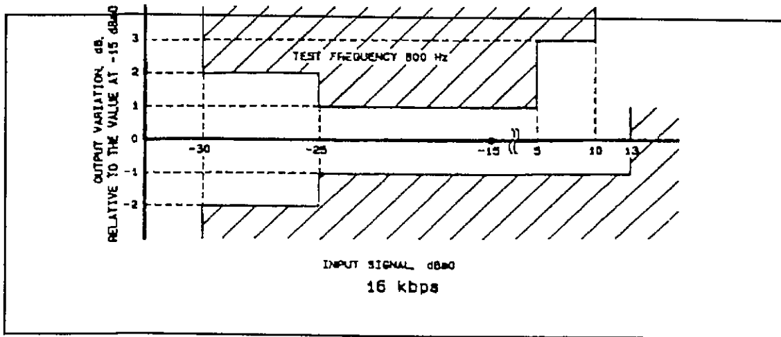
Figure F-5a. Variation of gain with input level for CVSD (16 kbps).
