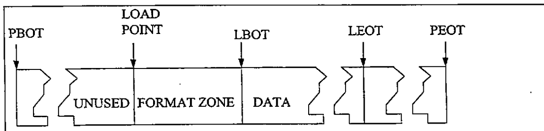
Figure 6-13. Tape cartridge layout.
