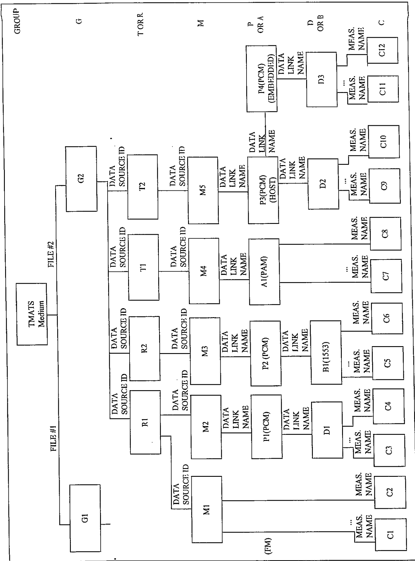
Figure 9-1. Group relationships.
