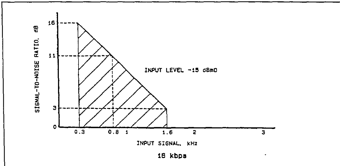
Figure F-7a. Signal to quantizing noise ratio versus frequency for CVSD (16 kbps).
