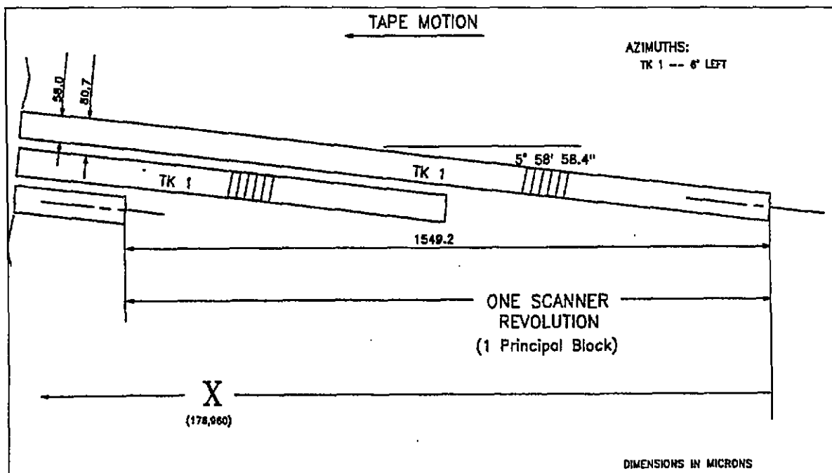
Figure 6-11. Helical track dimensions, E format.
