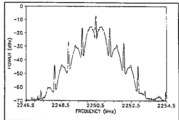
Figure A-4. Biφ PCM/PM signal.
