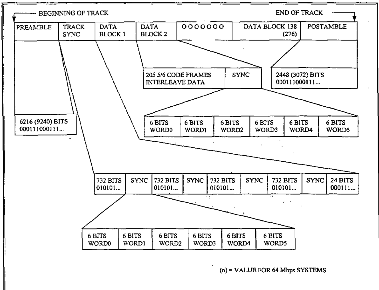
Figure 6-14. Helical Track Format.
