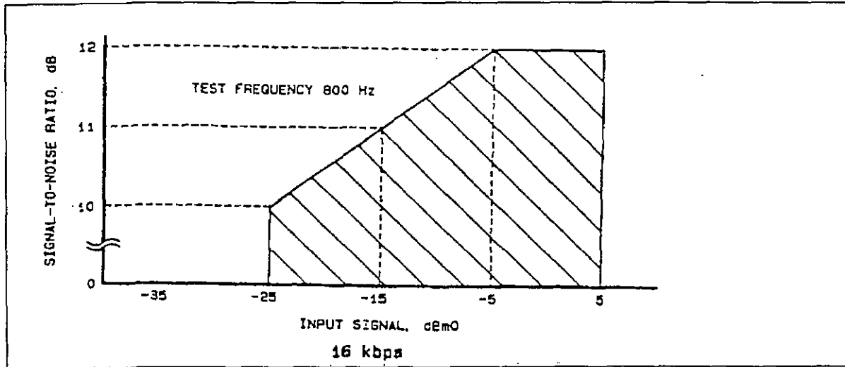
Figure F-6a. Signal to quantizing noise ratio versus input level for CVSD (16 kbps).
