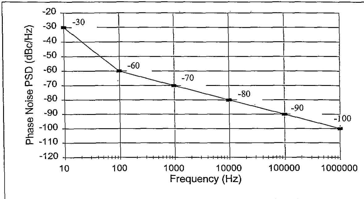
Figure 2-1. Continuous single sideband phase noise power spectral density.
